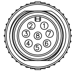
Pin Assignments Front View Conn.1&Conn.2
