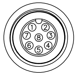
Pin Assignments Front View Conn.3
