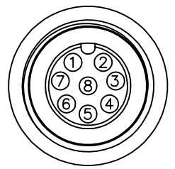
Pin Assignments Front View Conn.1&Conn.3
