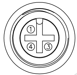
Conn.1 & Conn.2 Pin Assignments Front View
