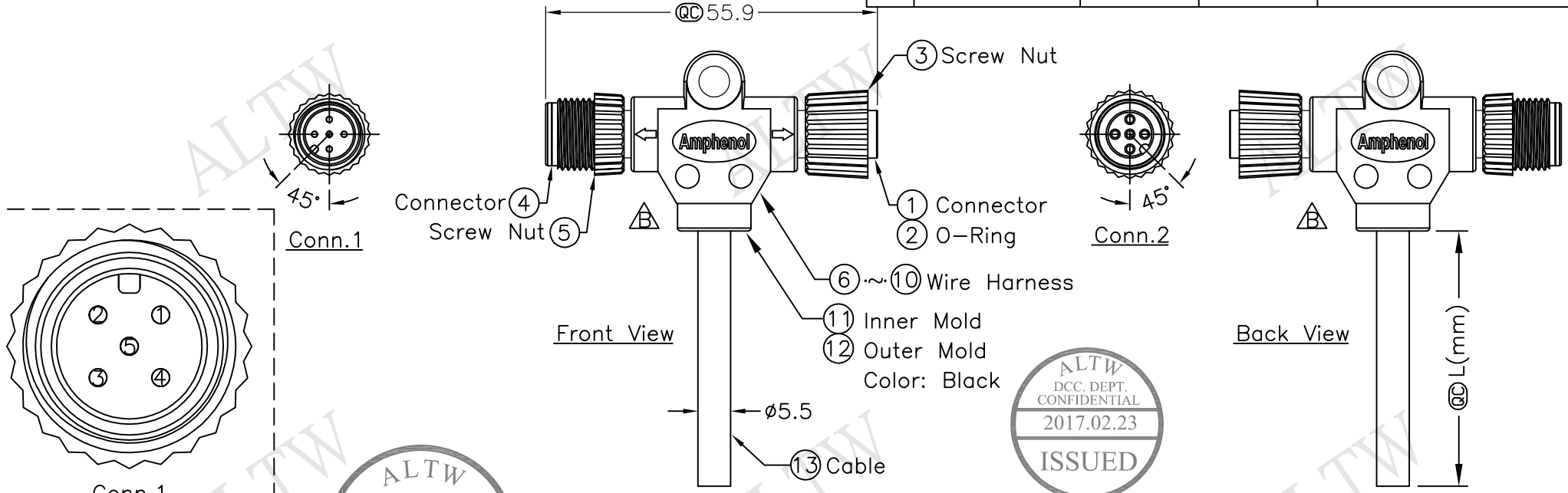
Conn.1 Pin Assignments Front View
