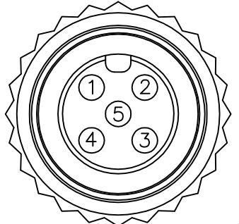
Conn.2 Pin Assignments Front View
