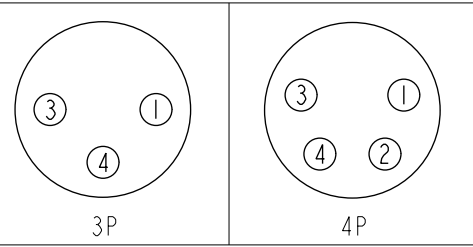
△E Pin Assignments Front View
