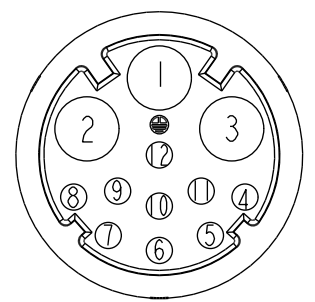
C1 & C2 Pin Assignments Front View
