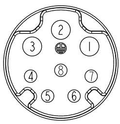
C1 & C2 Pin Assignments Front View
