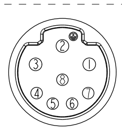
C2 Pin Assignments Front View
