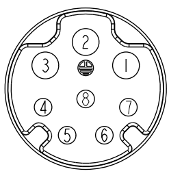
C1 Pin Assignments Front View
