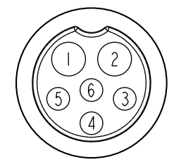
C2 Pin Assignments Front View
